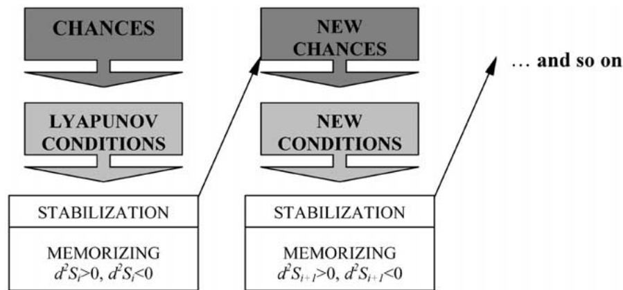
Figure 5. The dynamics of the self-organizing process (modified from Khazen, 2000). Legend: d^2S_i – entropy/information increment.
