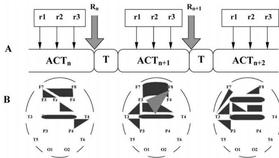
Figure 6. The schematic illustration of the behavioral/cognitive continuum (A modified from Alexandrov, 1999).
