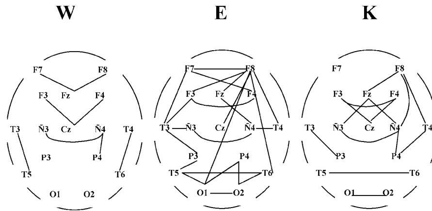
Figure 2. Maps of the operational synchrony configurations for pair EEG combinations during memory task periods, which were presented in chronological sequence: W – waiting period, E – encoding period, K – keeping-in-mind period. The lines indicate cases of upper-threshold IOS ( IOS > 2, p < 0.001 ).
