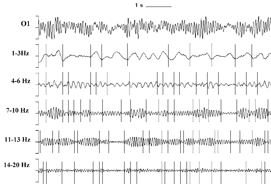
Figure 4. An example of RTP in basic frequency bands within the same EEG channel. Note that there is some sort of RTP synchronization between different oscillations within the same EEG signal.
