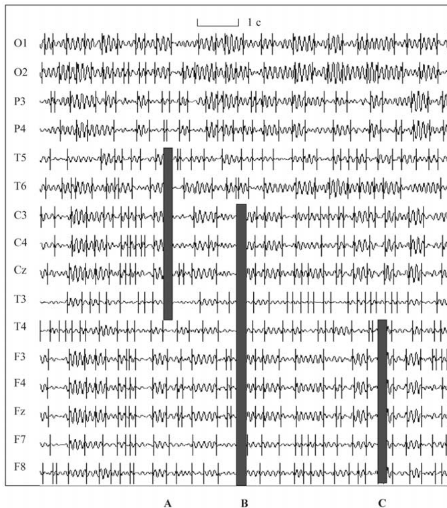
Figure 1. Typical fragment of 16-channel EEG record (filtered in alpha band diapason: 7–13 Hz) with automatically detected rapid transition processes (RTP). “A”, “B” and “C” illustrate some cases of RTP coincidence between different EEG channels.
