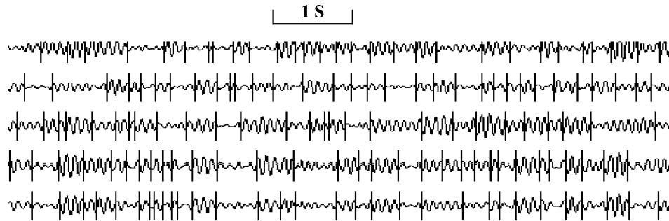
Fig. 1. Typical example of EEG channels with automatically detected rapid transitional processes (RTP). Note that the length of RTP is so brief that it appears to have almost zero duration in the figure (shown as vertical lines). Figure illustrates an example of five EEG channels (from the bottom: O1, O2, P3, Pz, P4.) filtered in the alpha frequency band. Subject was in rest condition, eyes open. It can be seen that some RTPs in different EEG channels appeared temporally close.
