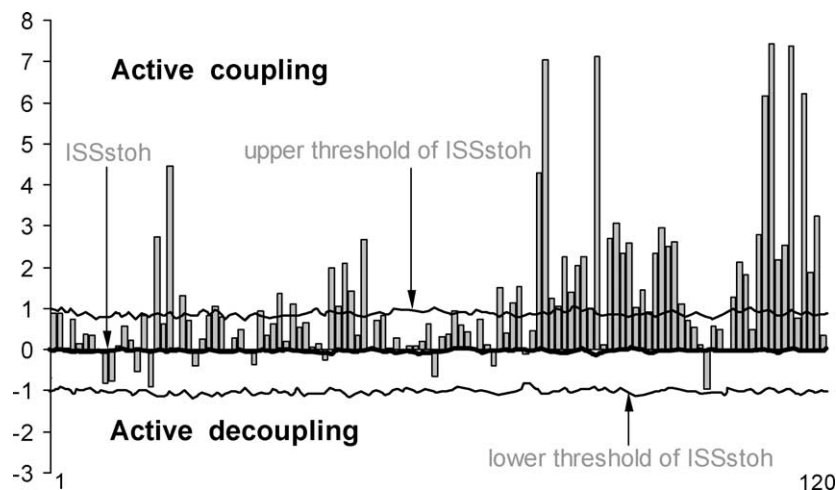
Fig. 2. Schematic illustration of the index of structural synchrony (ISS) and its stochastic levels. As an example, the calculations of ISS are shown for 16 EEG channels. The y-axis displays the ISS values found in the experiment (illustrated as gray bars). The x-axis displays the 120 possible pair combinations of 16 EEG channels (1 = O1–O2, 2 = O1–P3, 3 = O1–P4, 4 = O1–T5, ..., 115 = F4–Fz, 116 = F4–F7, 117 = F4–F8, 118 = Fz–F7, 119 = Fz–F8, 120 = F7–F8). Control subject is in rest condition, eyes closed. Figure is reproduced from the Fingelkurts et al. 2004, Human Brain Mapping ©.
